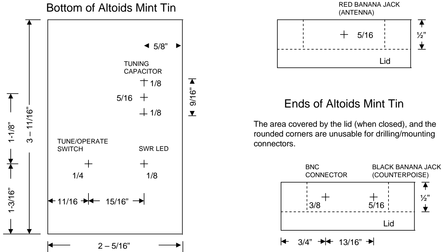
Hole Drilling Guide
